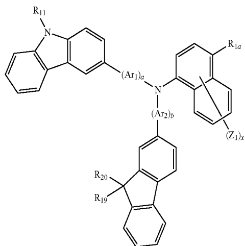
Formula 2B
