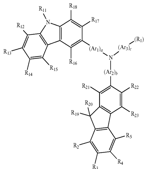
Formula 2
