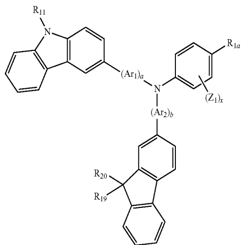
Formula 2A
