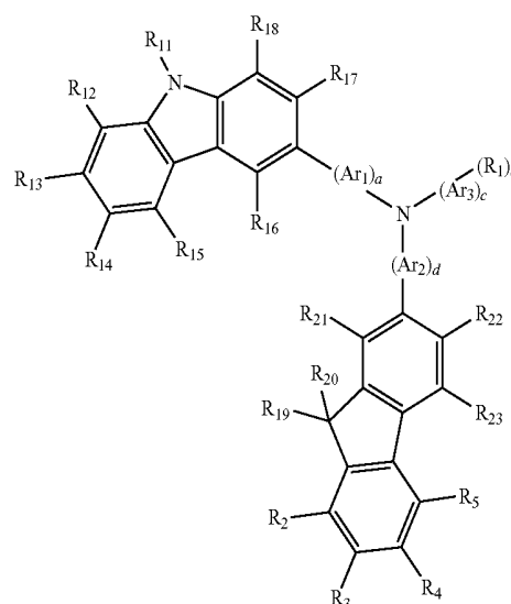
Formula 2
