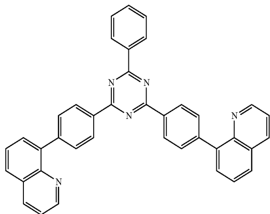
Comparative Example 2
