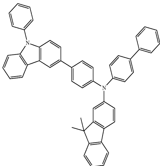
Compound 301
