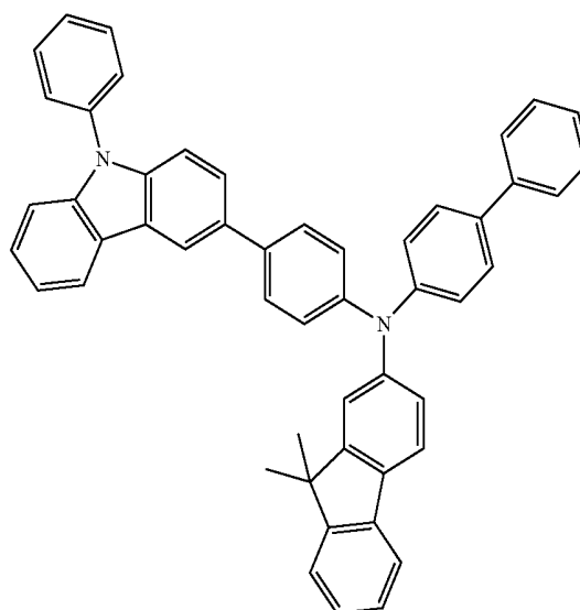
Compound 301
