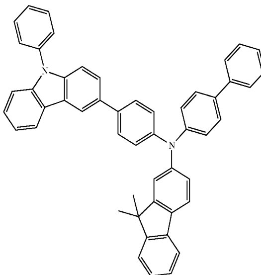
Compound 301
