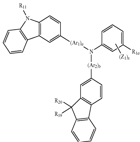
Formula 2C
