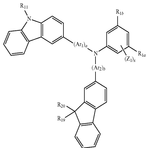
Formula 2D
