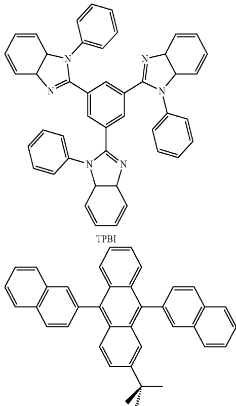
TBADN
